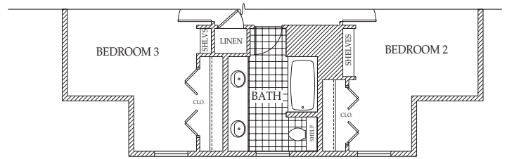
UPPER LEVEL FLOOR PLAN - ALT. ELEV. A
