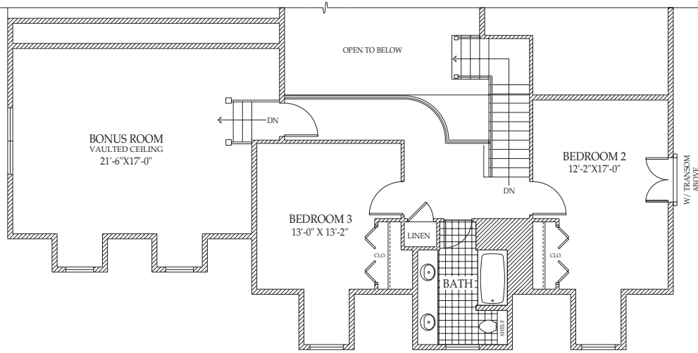
UPPER LEVEL FLOOR PLAN - OPT. BONUS RM. +555 S.F. *
